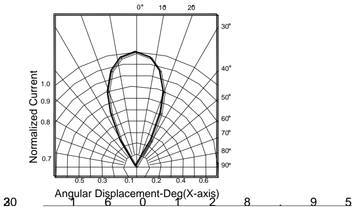
FIG.5 Light Current vs. Angular Displacement
