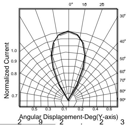
FIG.6 Light Current vs. Angular Displacement
